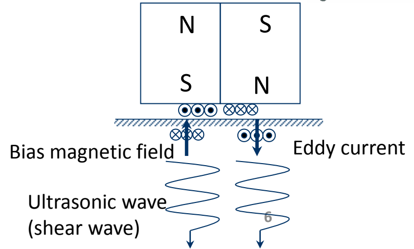
Eddy Current Field by Dual Probe
