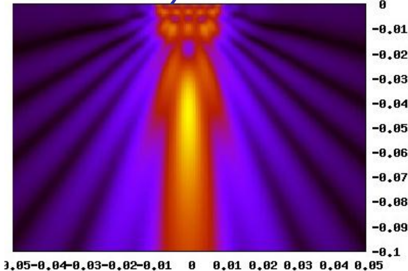
Sound Field by Dual Probe
