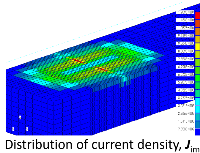
Eddy Current Field by Dual Probe
